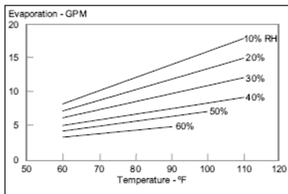
Figure-4 Evaporation rate for gas turbines 90-95% effective
